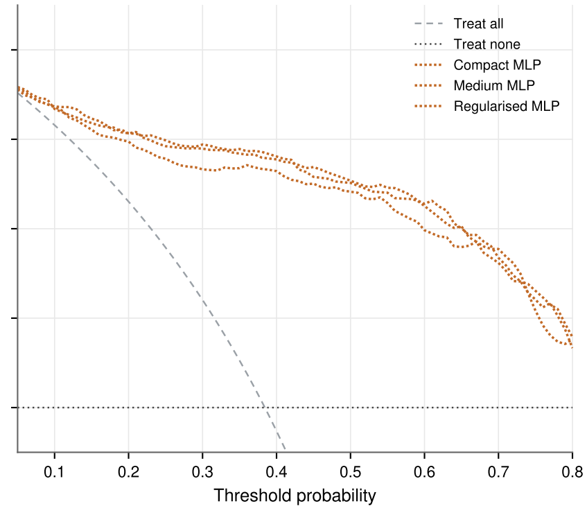
Neural networks
