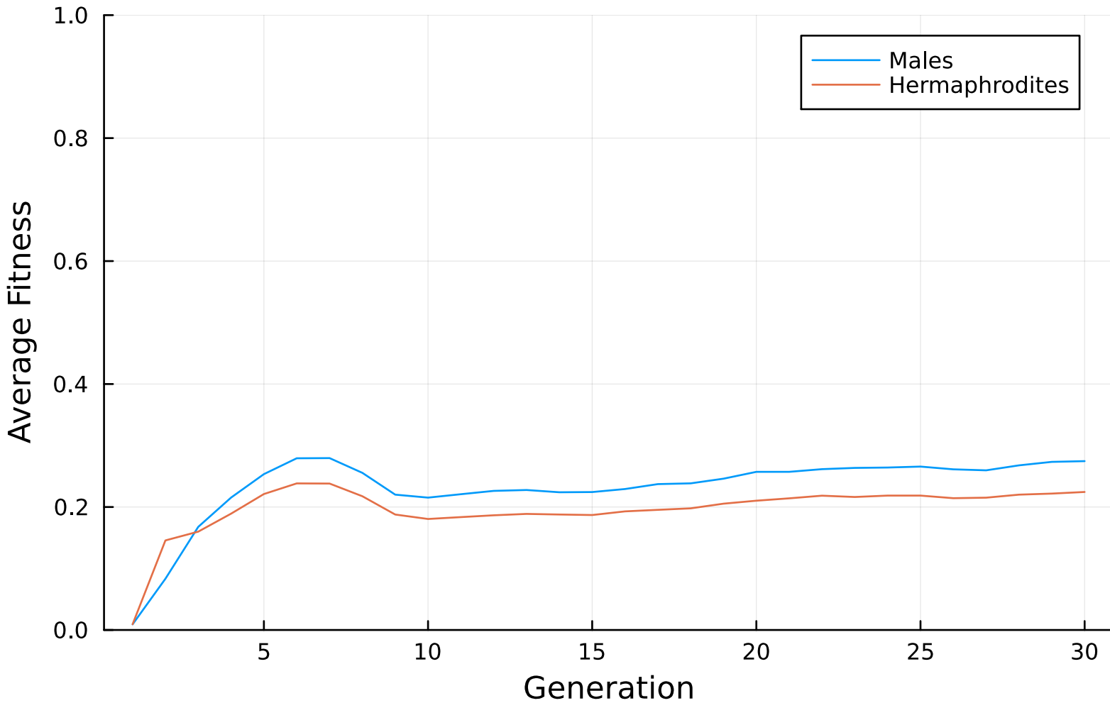
Male and Hermaphrodite Fitness, 1000 Replicates
