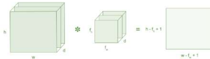
Figure 2: Image matrix multiplies kernel or filter matrix
