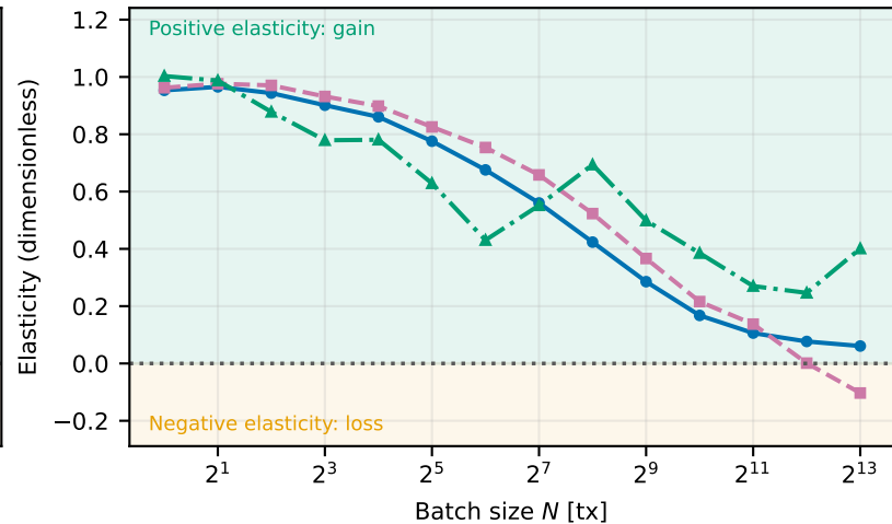
(b) snarkjs/prove
