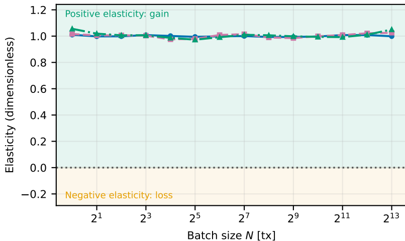
(c) verify
