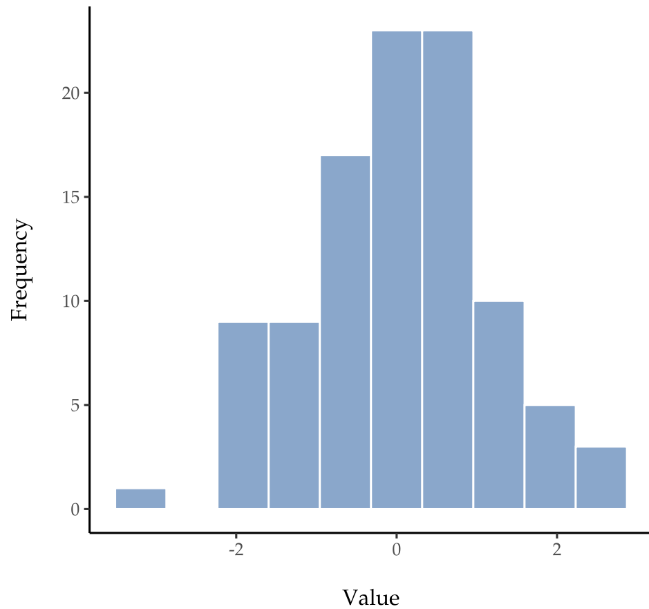
Normally Distributed Data
