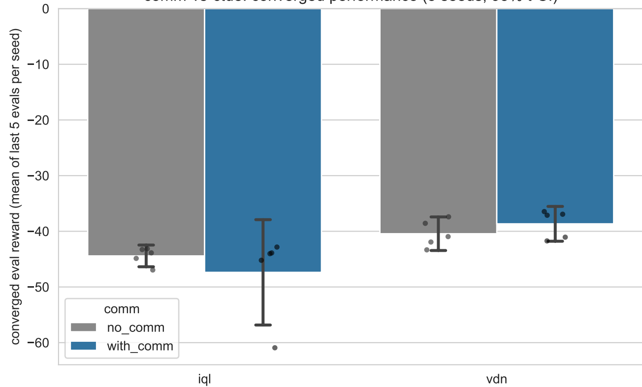
comm-vs-ctde: converged performance (5 seeds, 95% t-CI)
