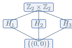
Subgroup lattice of \mathbb{Z}_2 \times \mathbb{Z}_2
