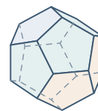
Dodecahedron
