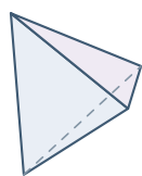
Tetrahedron
