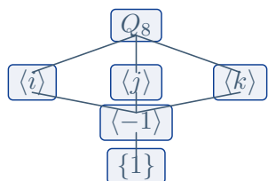
Subgroup lattice of Q_8
