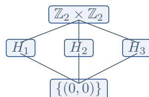
Subgroup lattice of \mathbb{Z}_2 \times \mathbb{Z}_2
