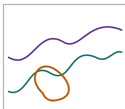
subtract the tangent plane random geometry is exposed
