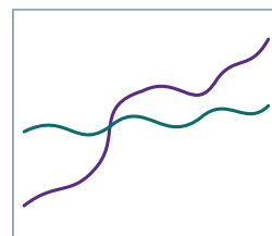
Kardar–Parisi–Zhang scaling directed landscape contours
