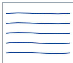
uncentred contours macroscopic shape dominates
