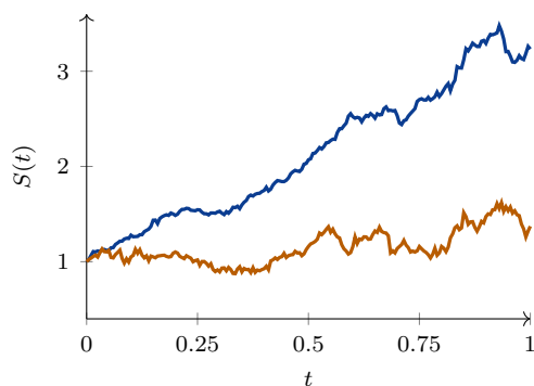
Sample paths of geometric Brownian motion
