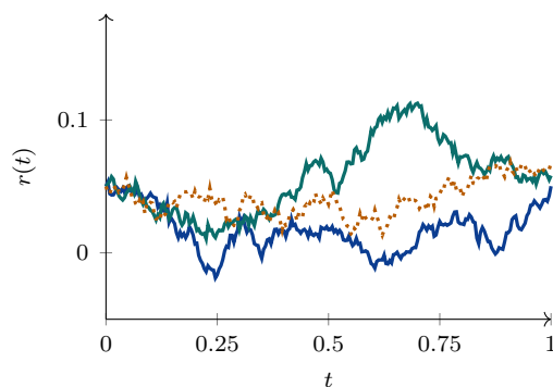
Sample paths of the Vasicek short rate
