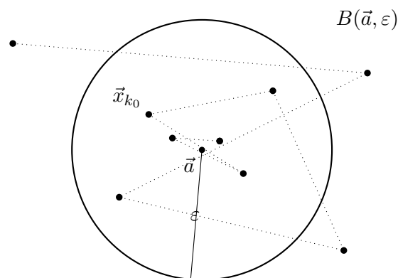
Figure 2: Tail of a sequence lying in an \varepsilon -ball around \vec{a} (from index k_0 onward).
