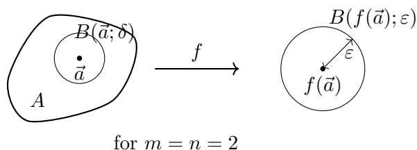
Figure 3: \varepsilon - \delta picture for continuity at \vec{a} : points in B(\vec{a}; \delta) map into B(f(\vec{a}); \varepsilon) .
