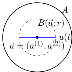
Figure 9: The case n = 2 , i = 2 : fixing the first coordinate and varying t to form u(t) = f(a^{(1)}, t) .
