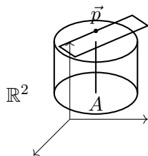
Figure 10: Geometric setup used in the argument: a point and an intersecting plane inside the ambient set A .
