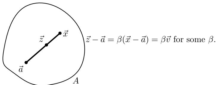
Figure 12: A point \vec{z} on the segment from \vec{a} to \vec{x} , with \vec{z} - \vec{a} = \beta(\vec{x} - \vec{a}) .
