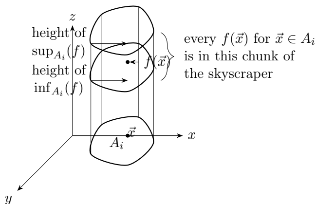
Figure 14: Skyscraper picture over A_i : values of f(\vec{x}) lie between \inf_{A_i} f and \sup_{A_i} f .
