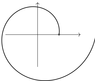
Figure 6: The spiral path f(t) = e^t(\cos(2\pi t), \sin(2\pi t)) for t \in [0, 1] .
