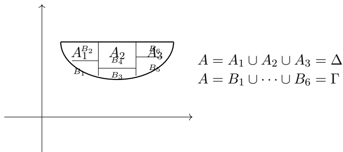
Figure 13: Two partitions \Delta and \Gamma of the same region A .
