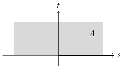
Figure 8: The set A = \{(s, t) \mid t > 0\} \cup \{(s, 0) \mid s \geq 0\} in the (s, t) -plane.
