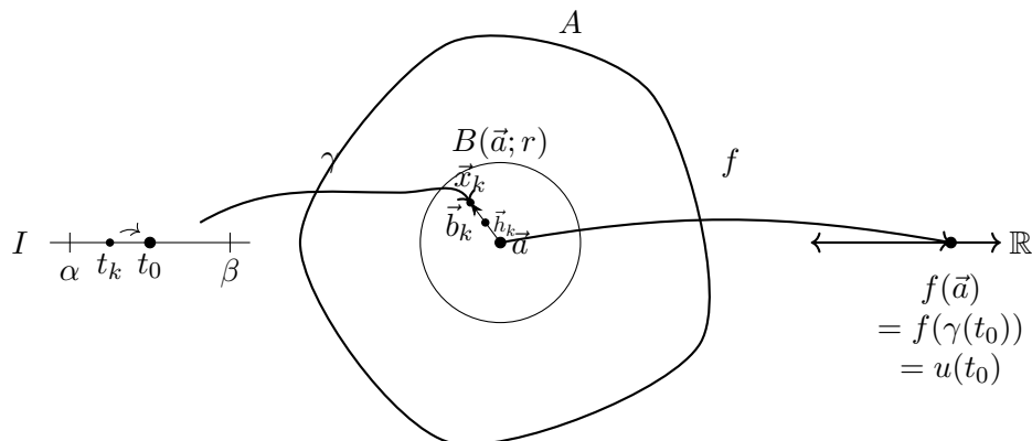
Figure 11: A path \gamma through \vec{a} = \gamma(t_0) and the induced one-variable function u = f \circ \gamma .
