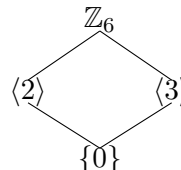
Subgroup lattice of \mathbb{Z}_6
