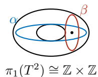
Loops on the torus
