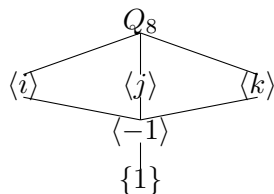
Subgroup lattice of Q_8
