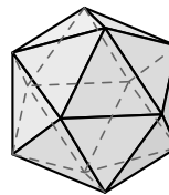
Icosahedron
