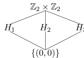
Subgroup lattice of \mathbb{Z}_2 \times \mathbb{Z}_2
