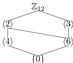
Subgroup lattice of \mathbb{Z}_{12}
