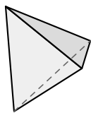
Tetrahedron
