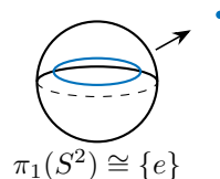
Loops on the sphere
