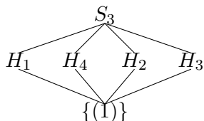
Subgroup lattice of S_3
