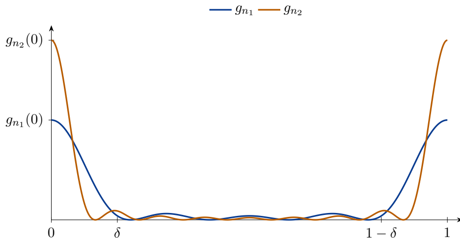
Figure 1: A summability kernel: g_{n_1} (in blue) and g_{n_2} (in orange) on \mathbb{T} , where n_1 < n_2 .
