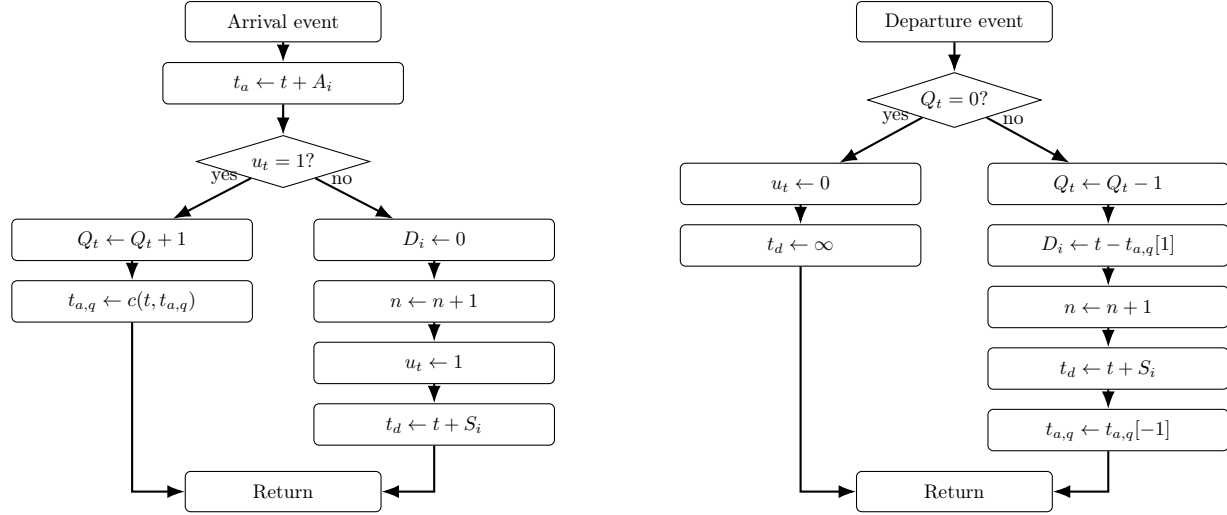
Figure 2: Flow charts for arrival and departure events in the next-event time-advance approach for an M/M/1 queue.
