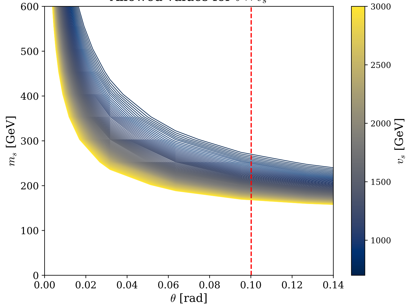
Allowed values for \theta \times v_s
