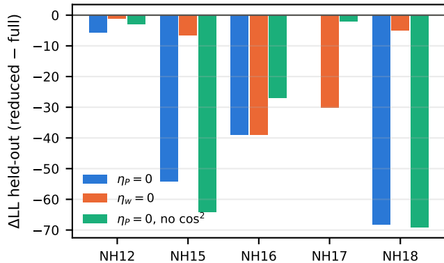
Held-out LL (even trials), reduced – full
