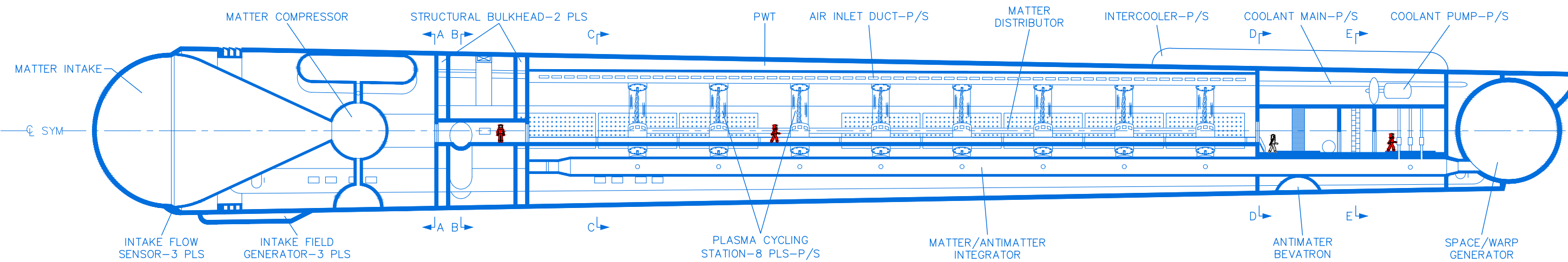
CL CUTAWAY PROFILE LOOKING TO STARBOARD (PORT SIDE UNIT SHOWN)
