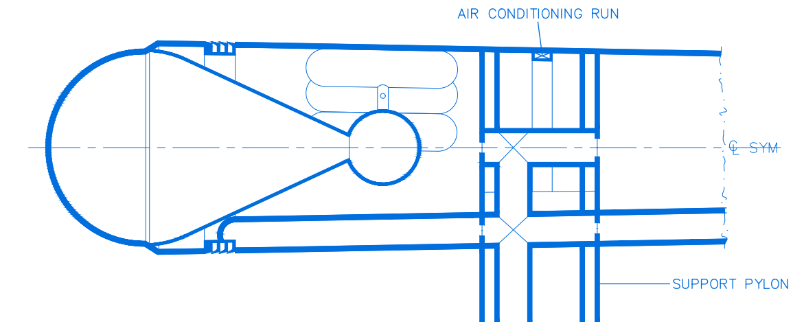
LONGITUDINAL CROSS-SECTION THROUGH CL OF PYLON
