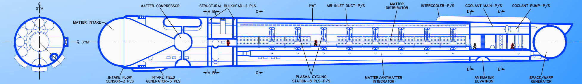
CUTAWAY PROFILE LOOKING TO STARBOARD (PORT SIDE UNIT SHOWN)
