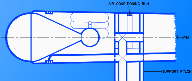
LONGITUDINAL CROSS-SECTION THROUGH C OF PYLON
