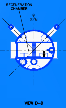
VIEW D-D
