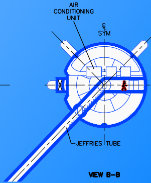
VIEW B-B
