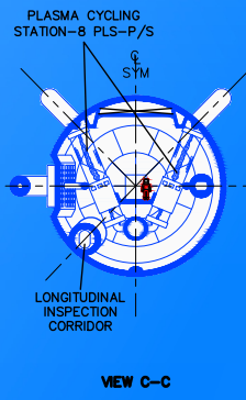
VIEW C-C
