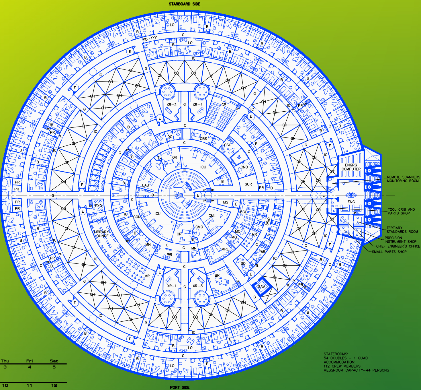
DECK 7. MAIN DECK
