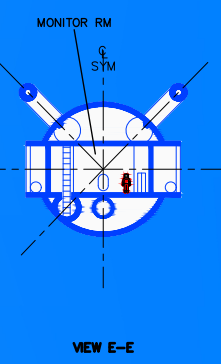
VIEW E-E
