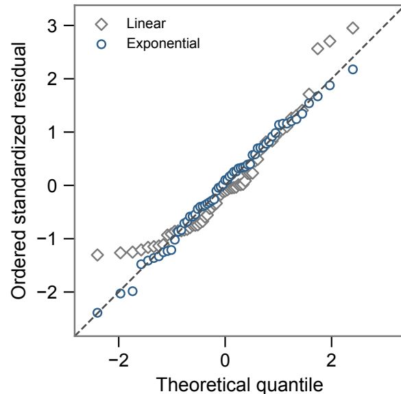
C. Normal Q-Q plots
