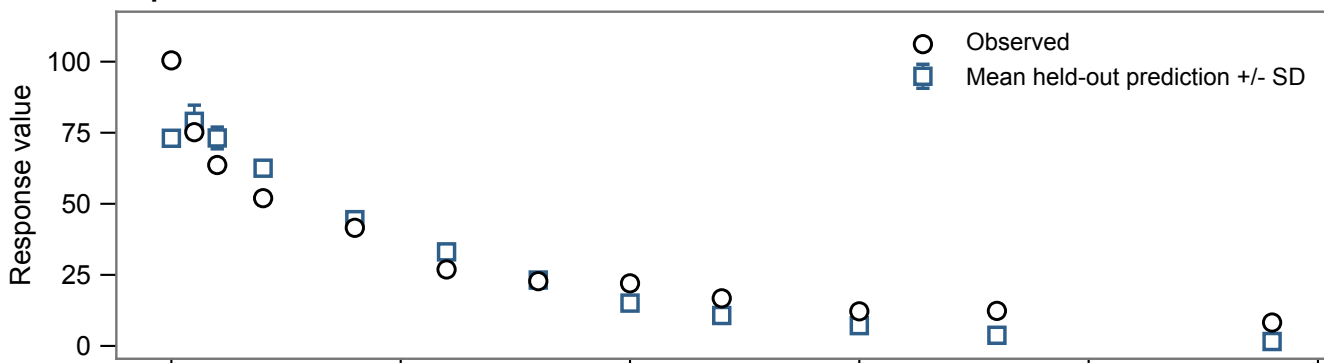
Exponential
