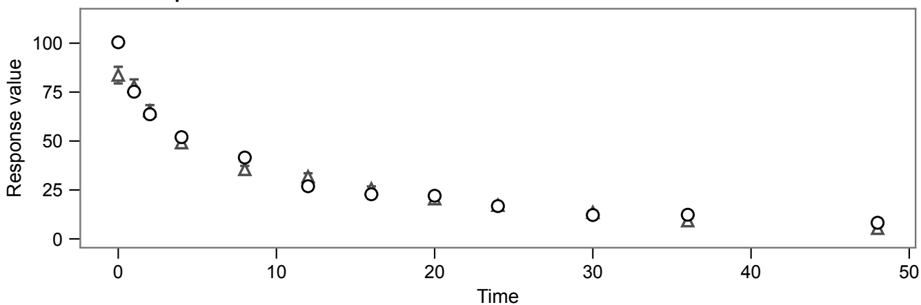
Double Exponential
