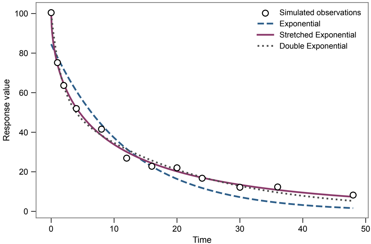
Candidate model fits to the same simulated dataset
