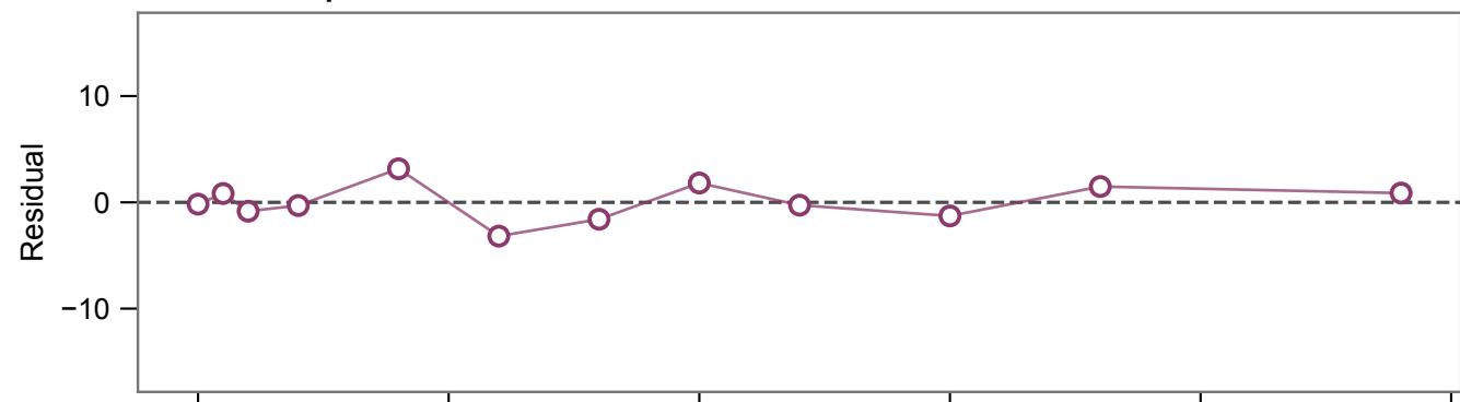
Double Exponential
