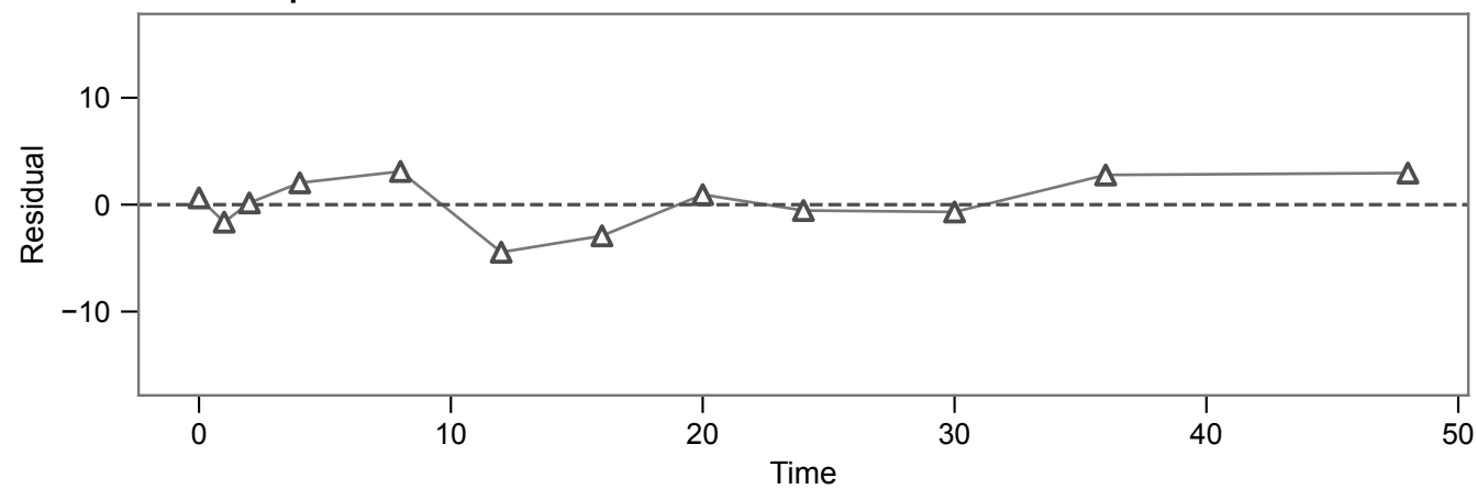
Double Exponential
