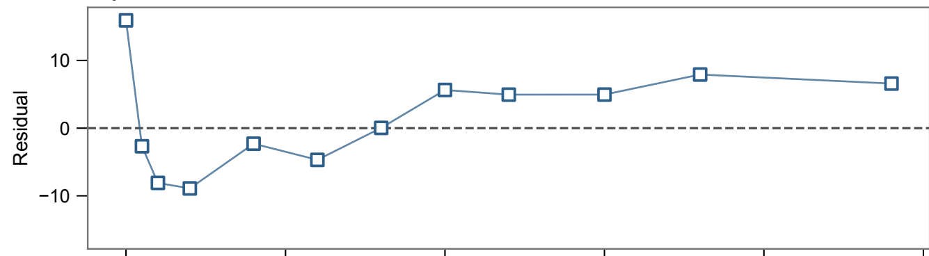
Stretched Exponential
