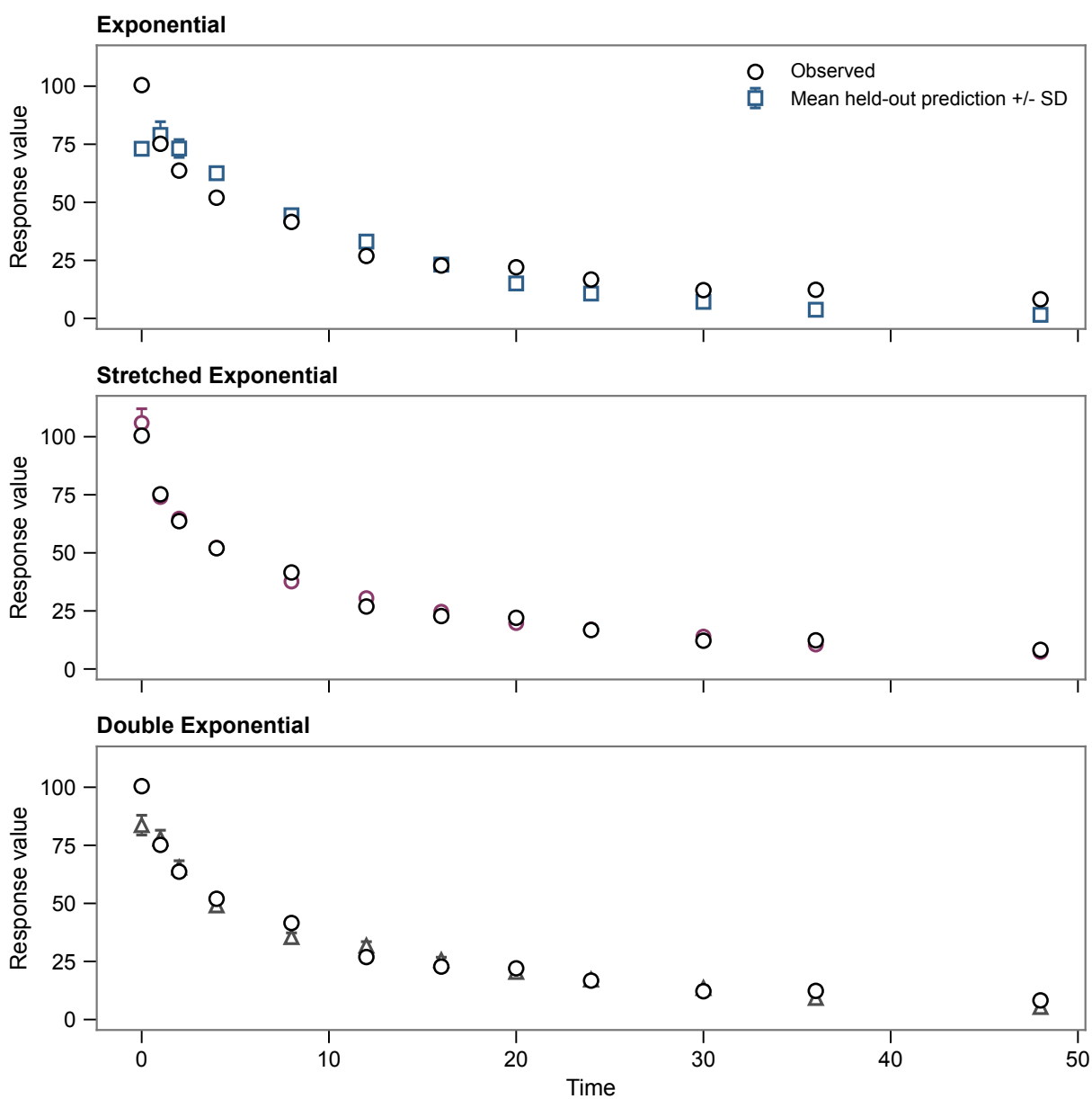
Figure 2: Observed responses and held-out predictions from shuffle-split cross-validation. Error bars show the standard deviation of the predictions obtained for each observation across splits in which it was omitted from fitting.
