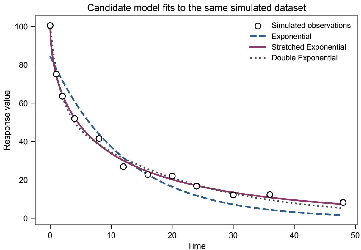
Figure 1: Candidate models fitted to the same simulated dataset.
