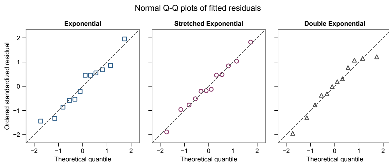
Figure 4: Normal Q-Q plots of standardized residuals.
