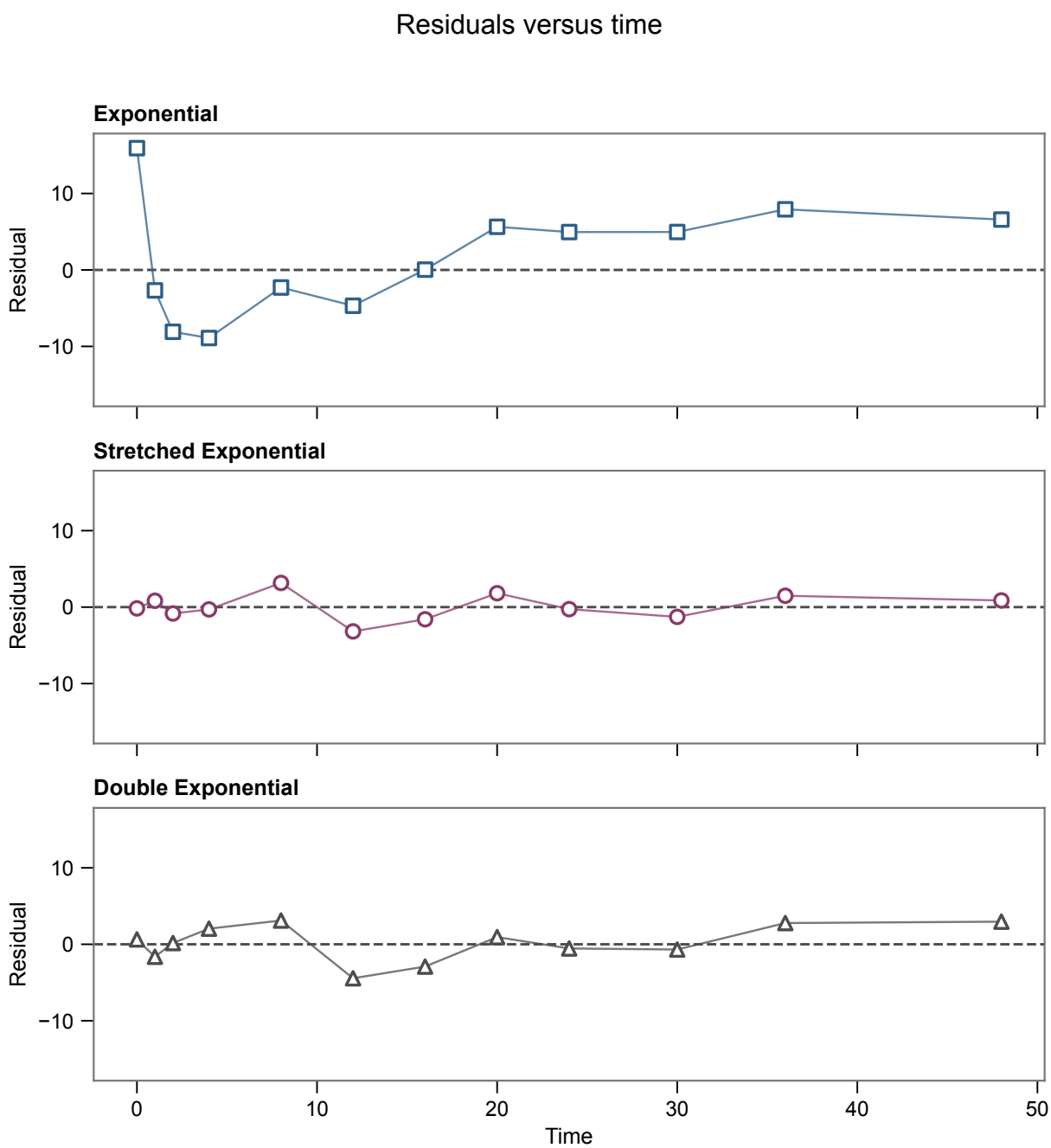
Figure 3: Residuals versus time for the three fitted models.
