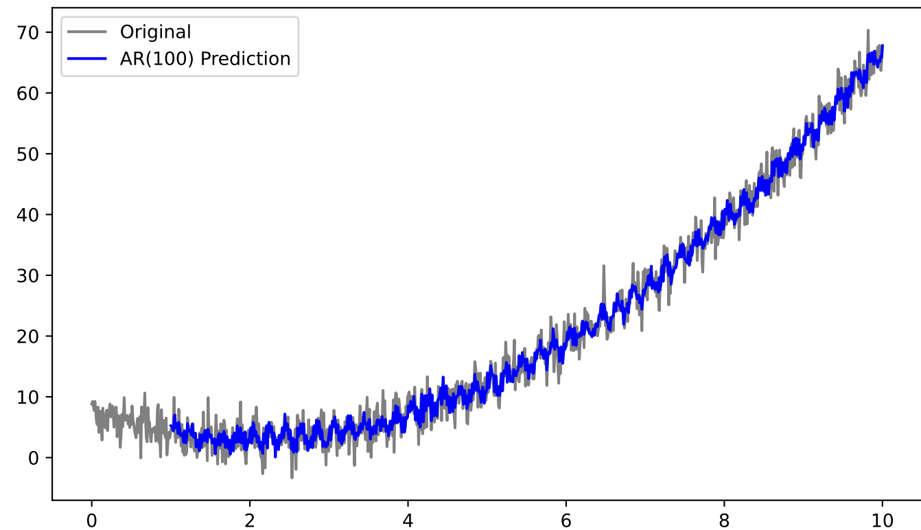
ARMA (statsmodels) Model for Time Series
