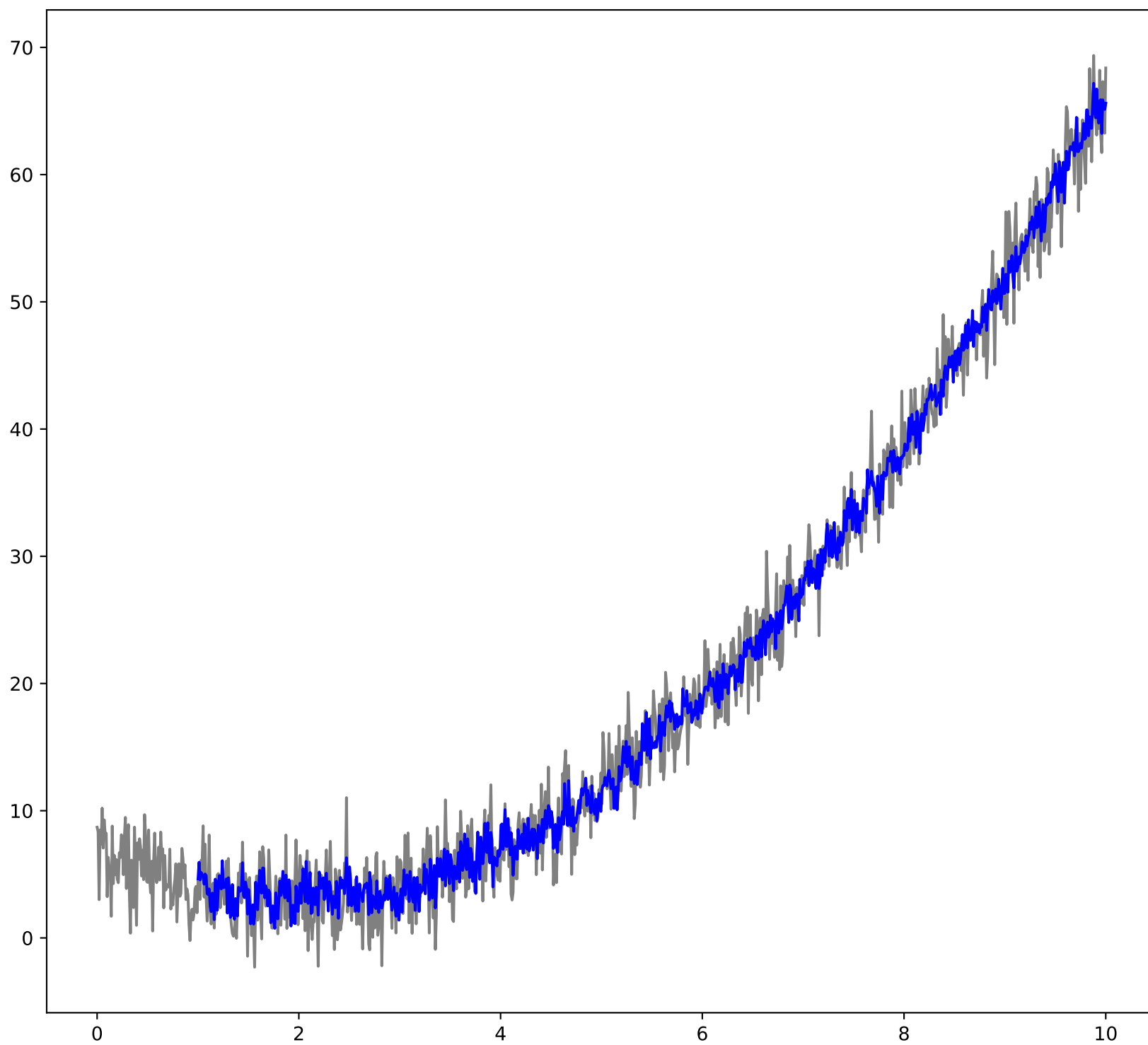
AR Model for Time Series
