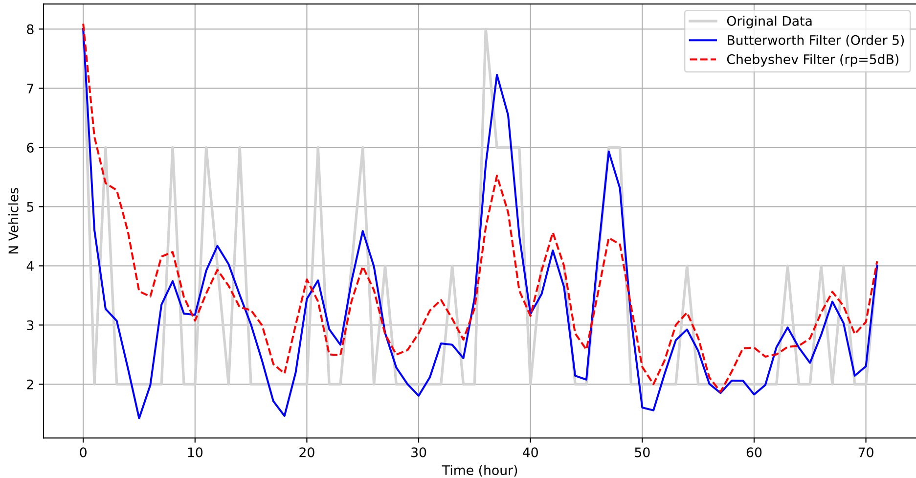
Butterworth vs Chebyshev
