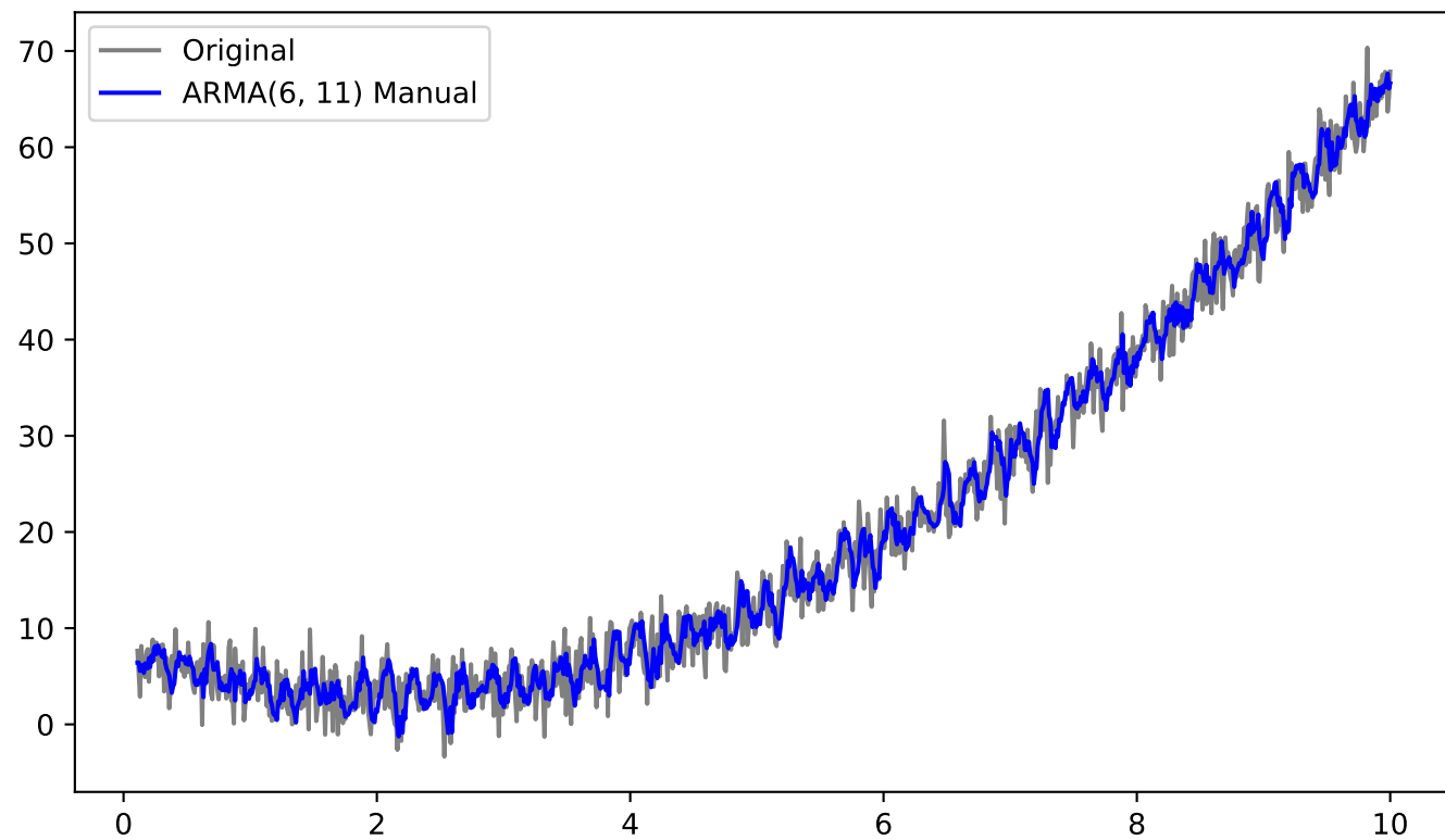
ARMA Model for Time Series
