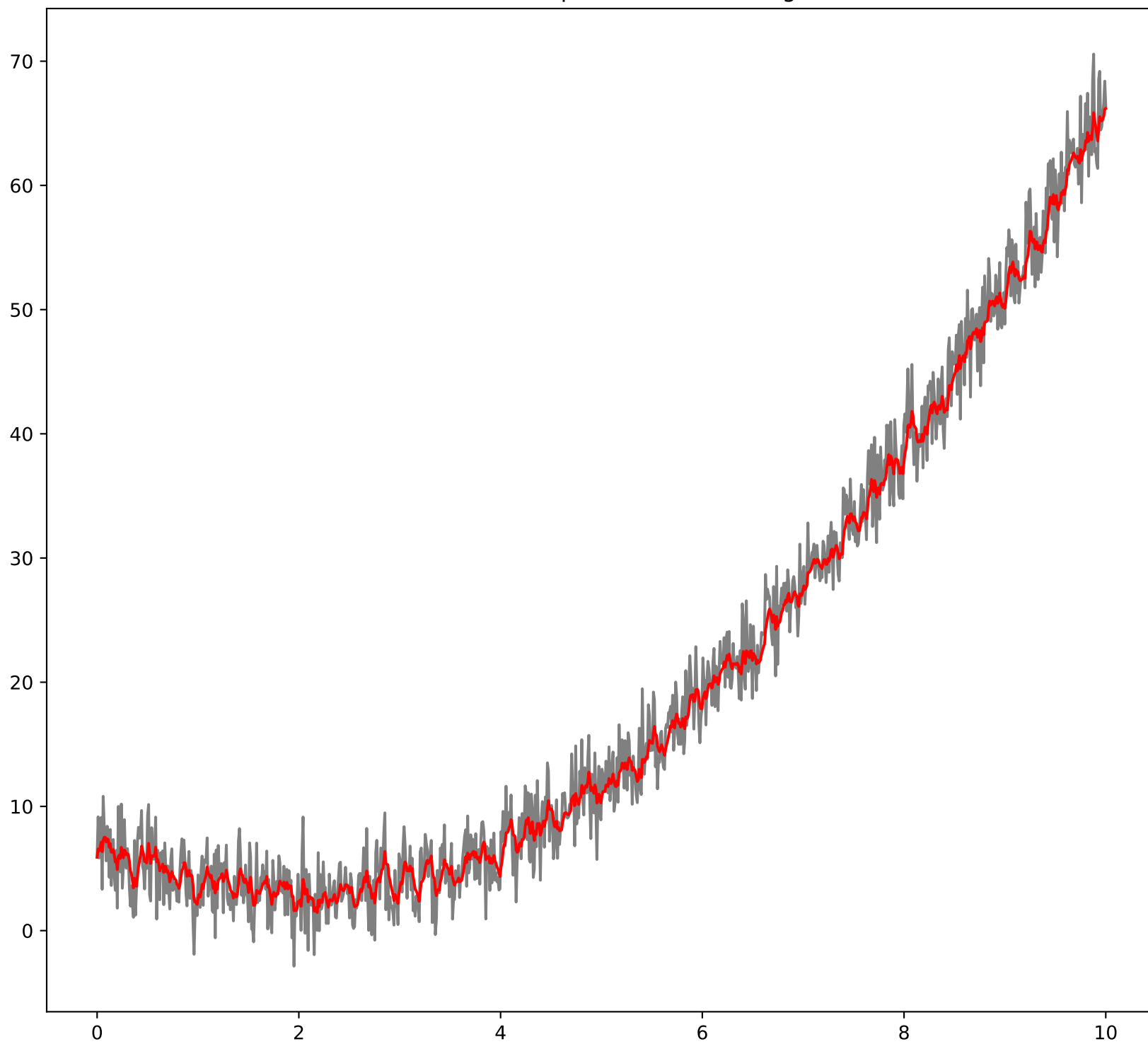
First Order Exponential Smoothing
