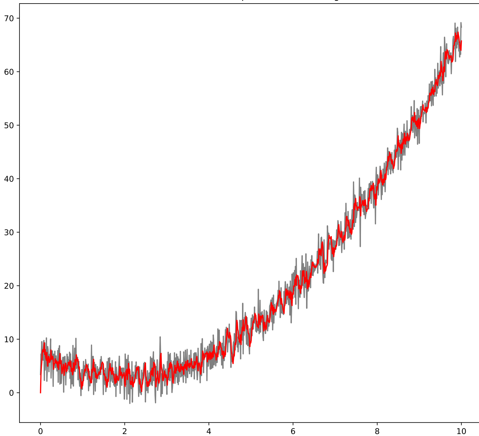
Second Order Exponential Smoothing
