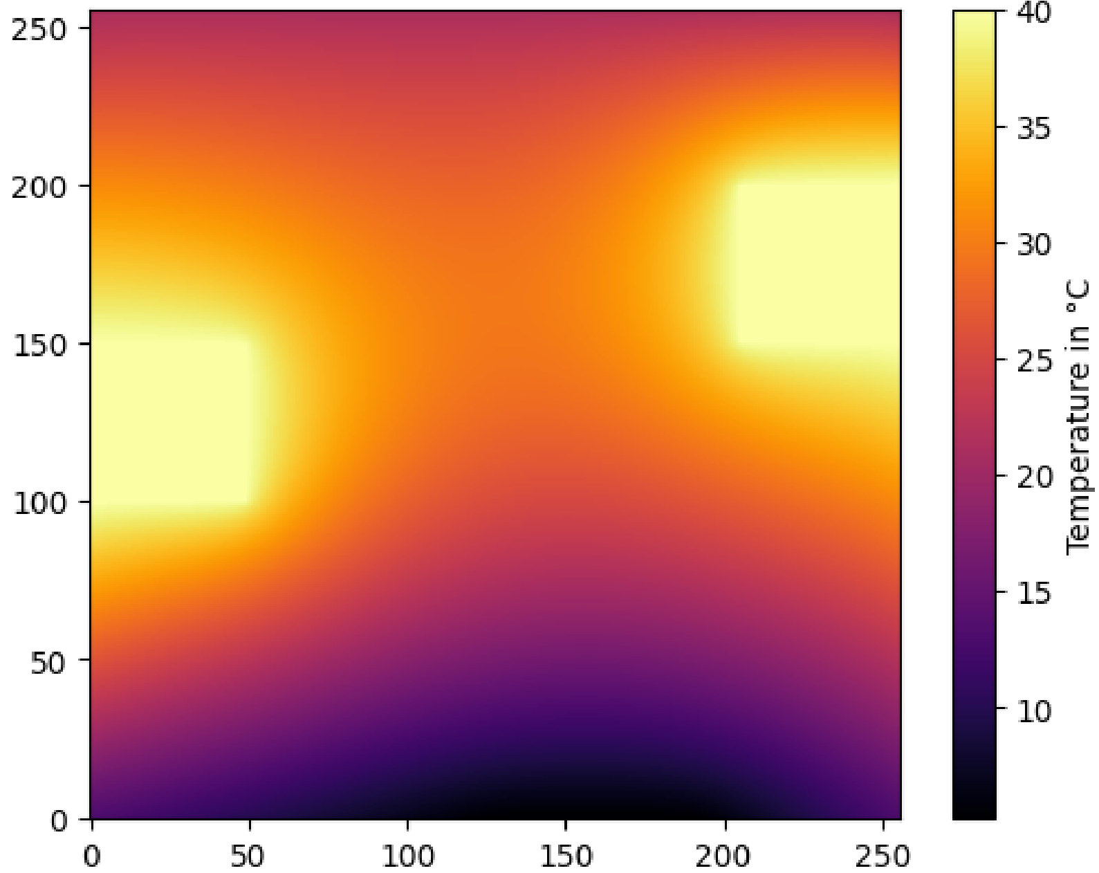
Stable heat distribution ( \Delta h = 0 ) with two heaters
