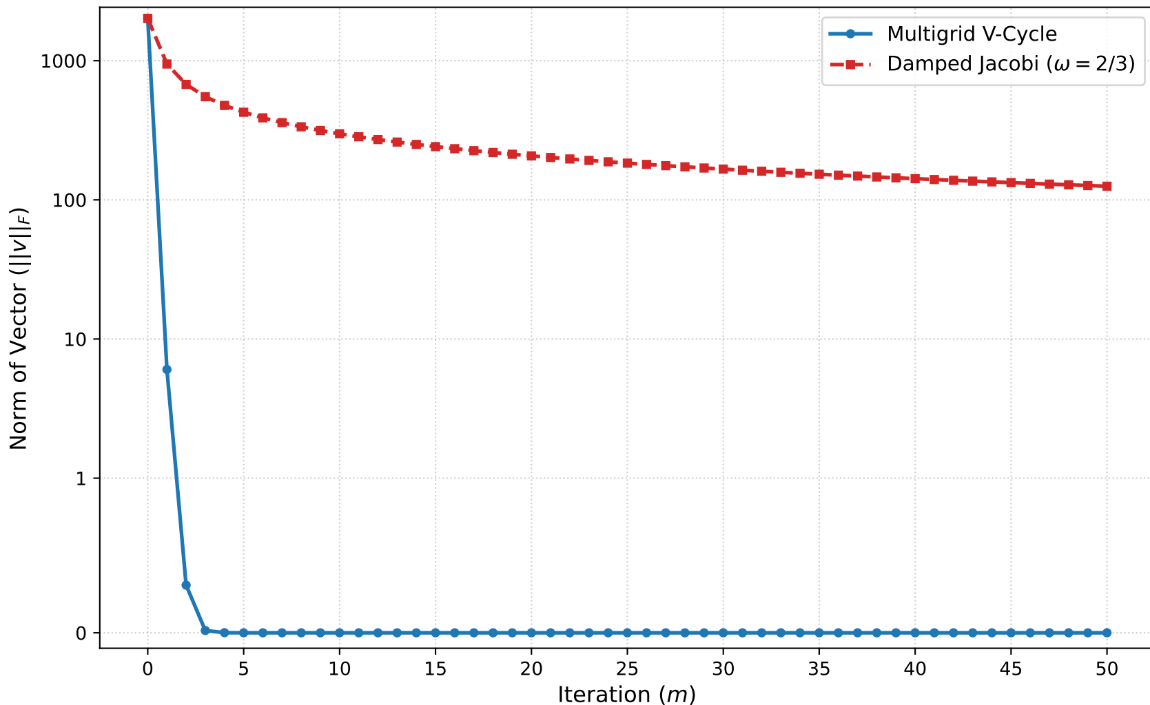
Convergence History: Multigrid V-Cycle vs. Damped Jacobi
