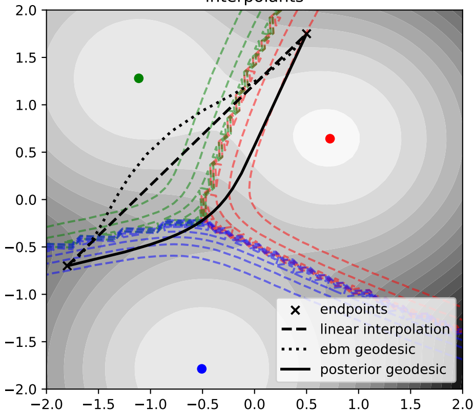
interpolants
