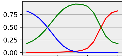
ebm geodesic
