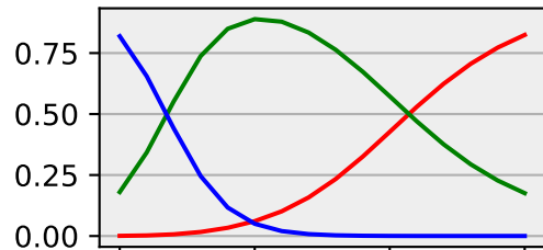
linear interpolation
