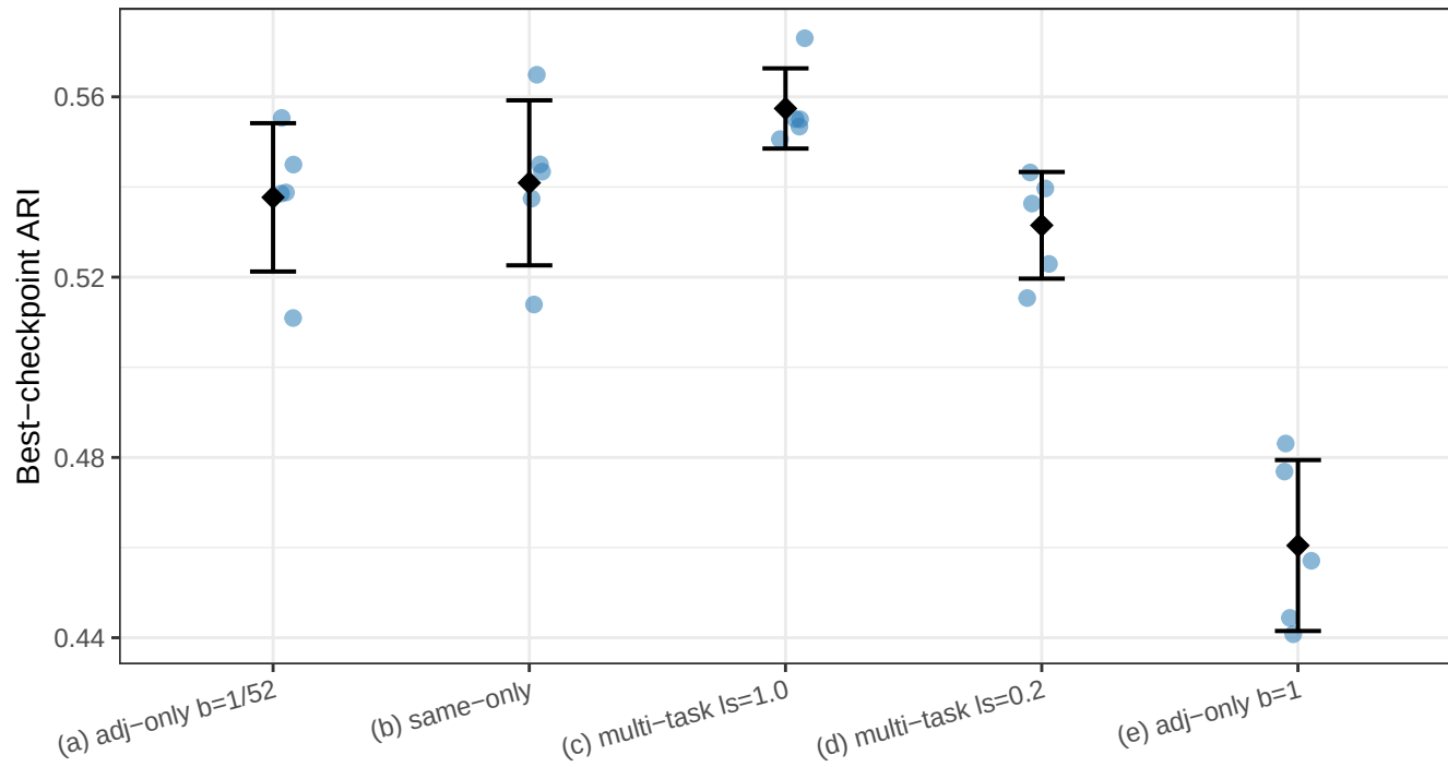
ARI by condition (n=5 seeds; diamond = mean, bar = \pm 1 SD)
