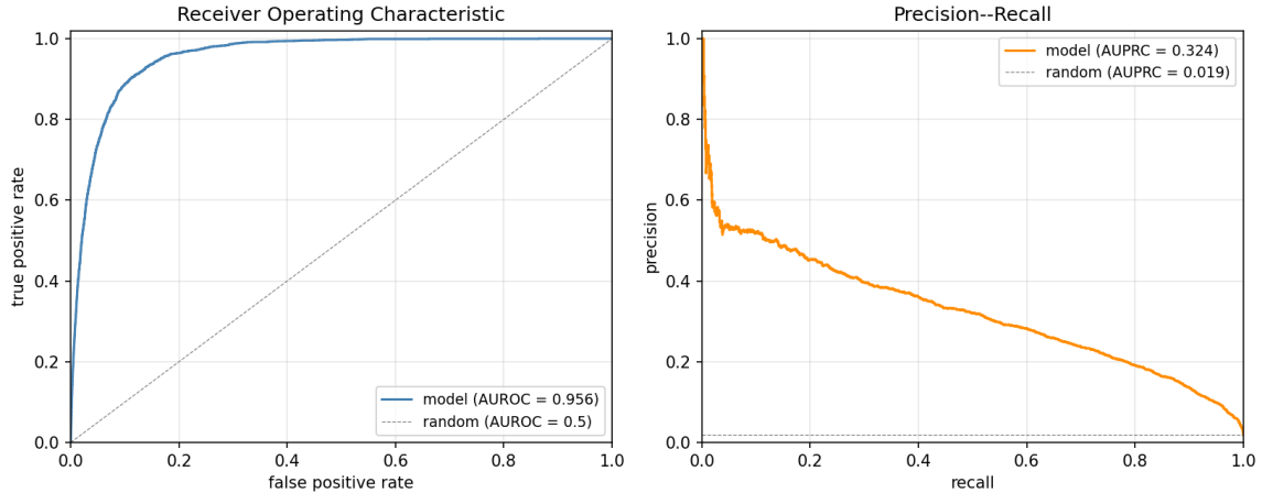
Figure 4: Threshold-free adjacency-prediction curves for the best checkpoint ( noise_seed_0 , \beta = 0.01923 , \lambda_{\text{adj}} = 1.0 , \lambda_{\text{same}} = 1.0 ). Curves aggregated over 10 fresh validation batches (127,200 pairs in total, with positive rate 0.0189). AUROC = 0.956 and AUPRC = 0.324; the AUPRC random baseline is the positive rate ( \approx 0.019 , dashed grey line).
