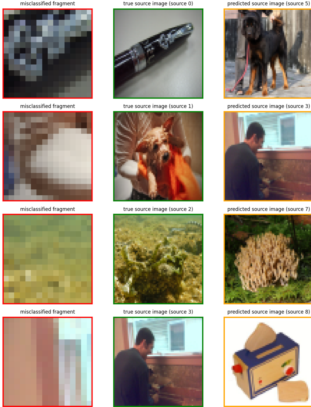
Figure 5: Selected misclassified fragments from the best checkpoint ( multitask_10 , best ARI = 0.570, \beta = 0.01923 , \lambda_{\text{adj}} = 1.0 , \lambda_{\text{same}} = 1.0 ). On the validation batch shown, 51 of 160 fragments were assigned to the wrong cluster after Hungarian matching of predicted to true labels. Each row shows: the misclassified fragment (left, red), the true source image (middle, green), and the source image the model assigned it to (right, orange).
