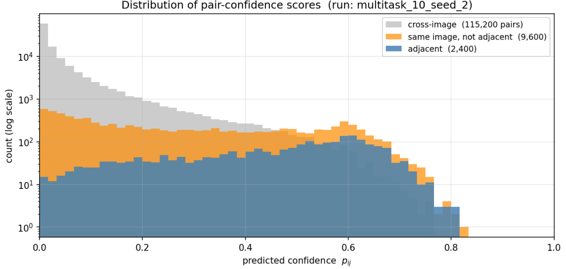
Figure 6: Distribution of the model’s per-pair confidence scores p_{ij} on 10 fresh validation batches ( multitask_10_seed_2 , \beta = 0.0192 , \lambda_{\text{adj}} = 1.0 , \lambda_{\text{same}} = 1.0 ). Pairs are split by their true class: adjacent (blue, 2,400 pairs), same source image but not adjacent (orange, 9,600), and cross-image (grey, 115,200). y-axis is logarithmic to make the rare classes visible.
