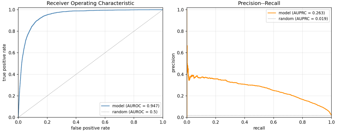
Figure 5: Threshold-free adjacency-prediction curves for the best checkpoint ( multitask_10_seed_2 , \beta = 0.01923 , \lambda_{\text{adj}} = 1.0 , \lambda_{\text{same}} = 1.0 ). Curves aggregated over 10 fresh validation batches (127,200 pairs in total, with positive rate 0.0189). AUROC = 0.947 and AUPRC = 0.263; the AUPRC random baseline is the positive rate ( \approx 0.019 , dashed grey line).
