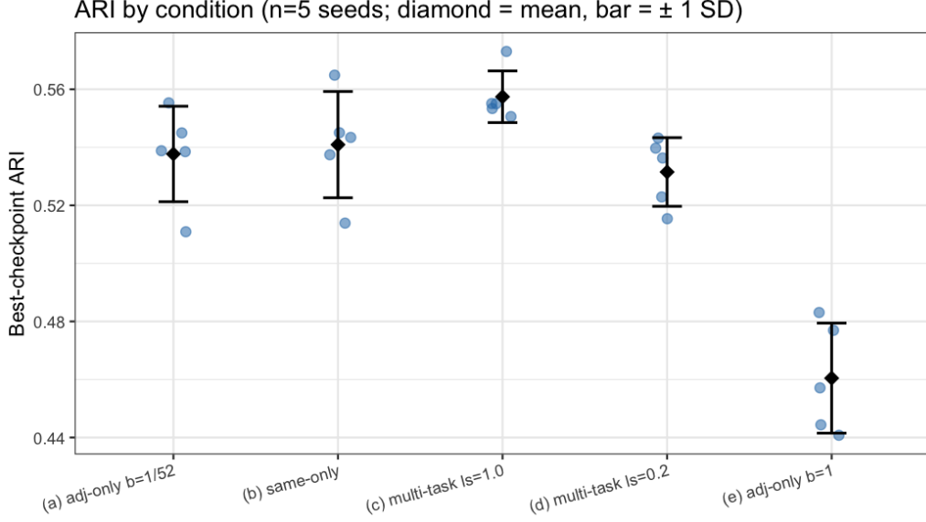
Figure 4: ARI per seed for each condition. Diamond = mean, bar = \pm 1 SD. Conditions (a)–(d) are tightly clustered; condition (e) ( \beta = 1 ) sits \sim 0.08 ARI lower.
