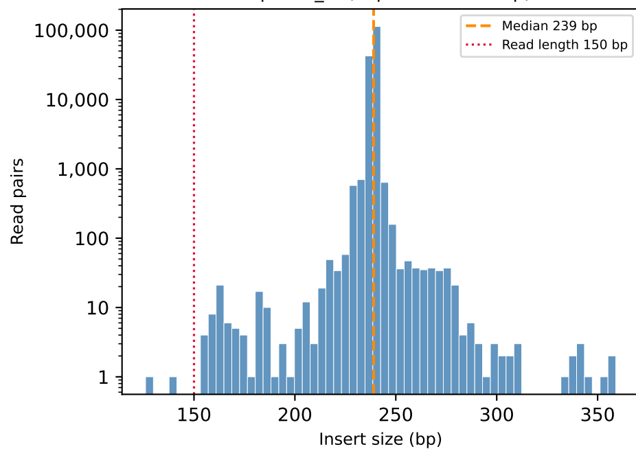
Amplicon_4 (expected \approx 238 bp)
