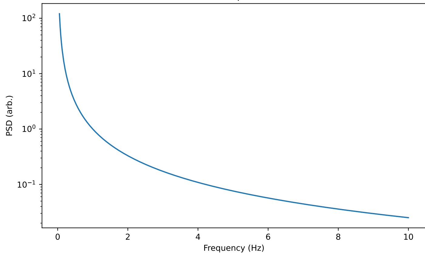
Position Spectrum
