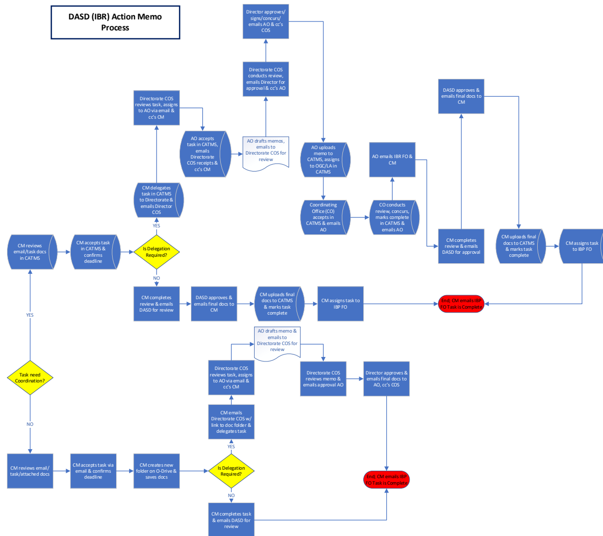
Figure 4: DASD IBR Action Memo Process
