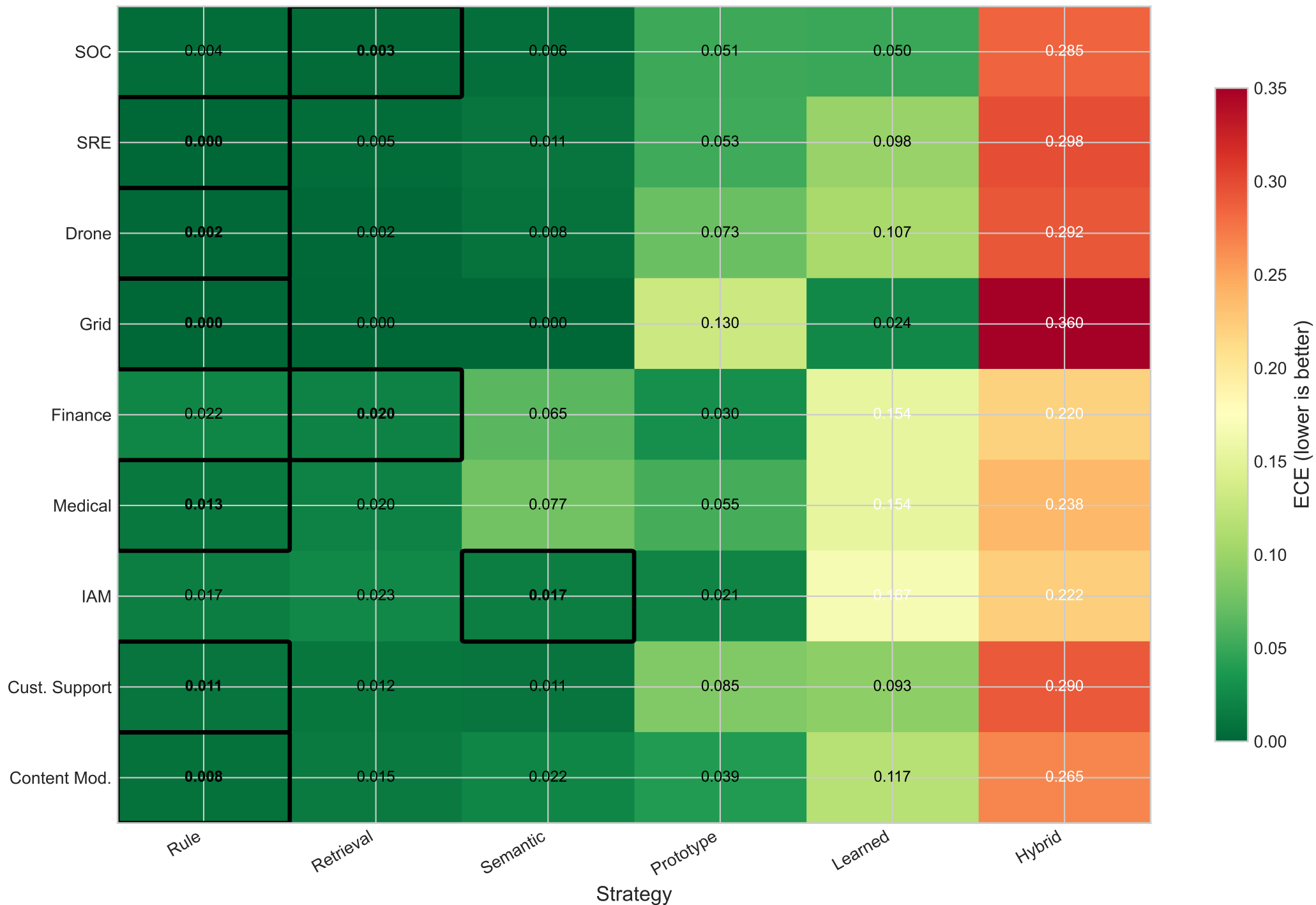
Expected Calibration Error by Domain and Strategy
