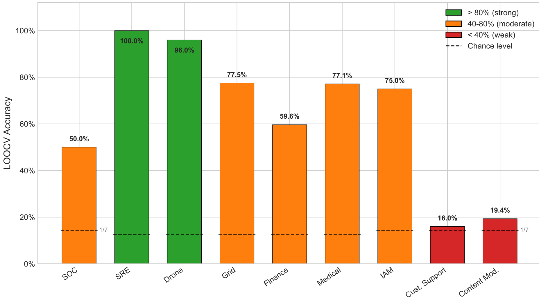
Compact Selector LOOCV Generalization Accuracy
