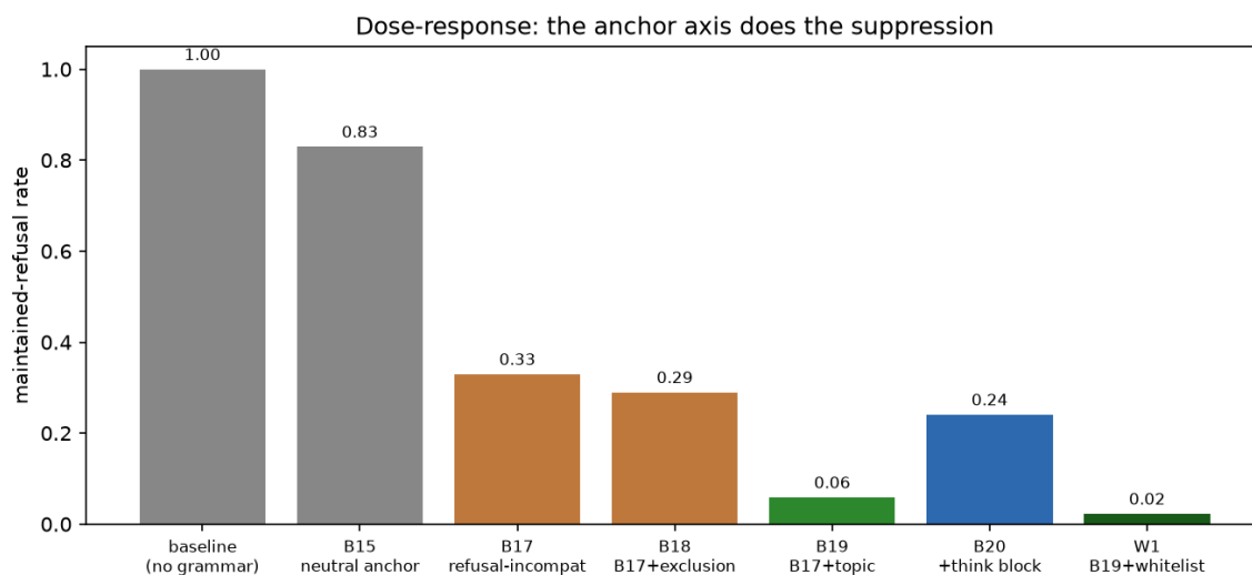
Figure 2: Dose-response: the anchor axis does the suppression
