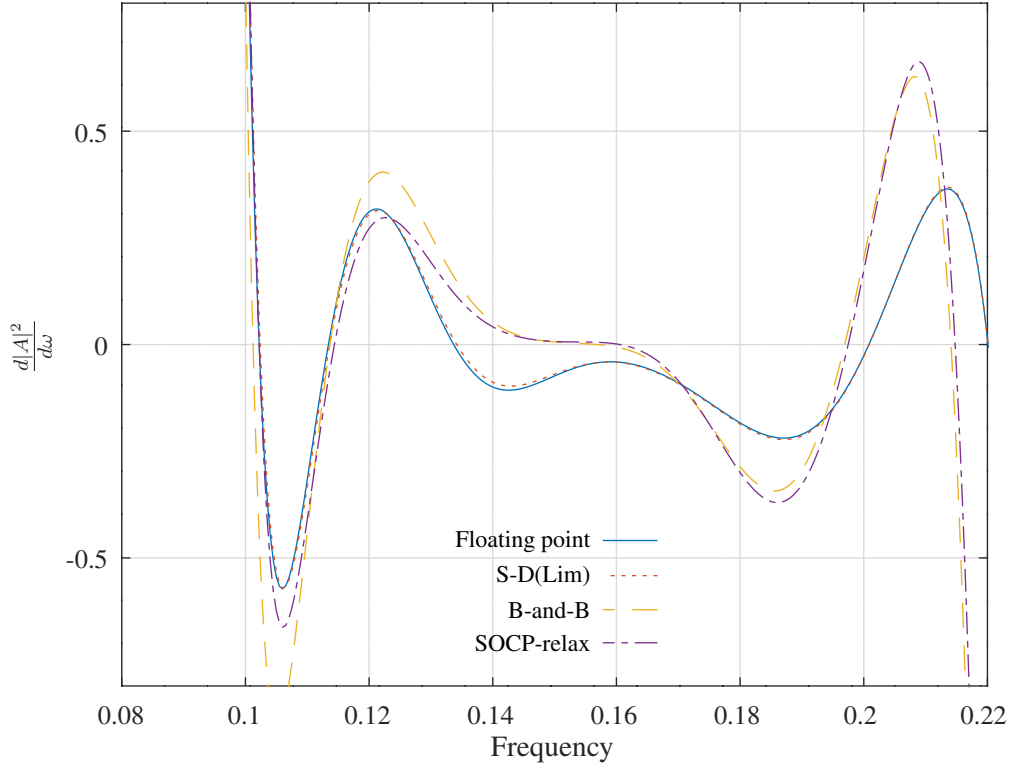
Figure 32: Comparison of the error in the pass band gradient of the squared magnitude response of a band pass Hilbert filter composed of a parallel doubly pipelined all pass filter band pass Hilbert filter in series with a parallel all pass anti-aliasing filter with floating point coefficients, 12-bit 3-signed-digit coefficients, and 12-bit signed-digit coefficients each having an average of 3-signed-digits allocated by the method of Lim et al. , found by branch-and-bound and SOCP relaxation search.
