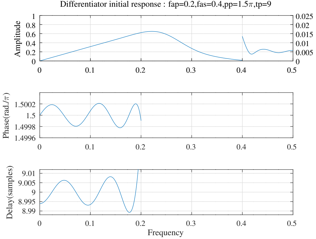
Figure 7: Amplitude, phase and group delay responses of an initial low pass differentiator filter composed of a Schur one-multiplier lattice correction filter with a denominator polynomial having terms only in z^{-2} in series with 1 - z^{-1} .
