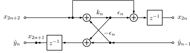
Figure 4: Doubly pipelined Schur one-multiplier all pass lattice section.
