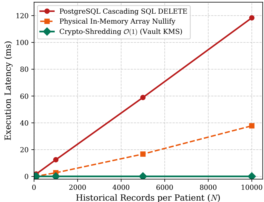
(a) Absolute Erasure Latency vs Record Count ( N )
