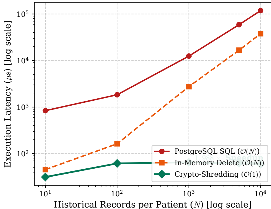
(b) Asymptotic Complexity (Log-Log Scale)
