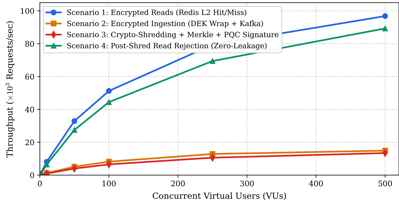
Macro System Throughput Across Concurrency Tiers (1 to 500 VUs)
