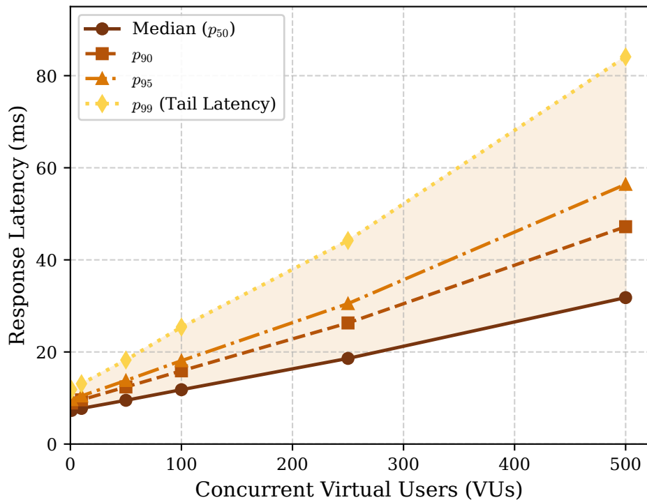
(b) Scenario 2: Encrypted Ingestion Latency (DEK Wrap + K)
