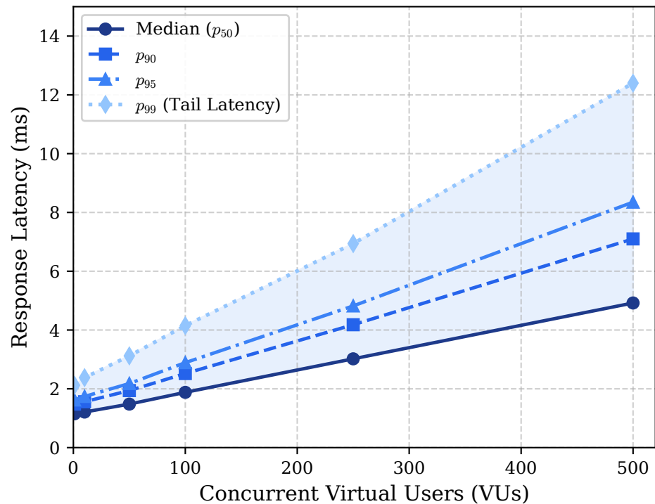
(a) Scenario 1: Encrypted Read Latency (Redis L2)
