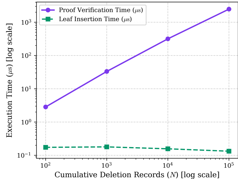
(a) Logarithmic ( \mathcal{O}(\log N) ) Verification Scaling
