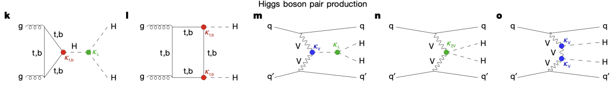
Figure 1.7. Feynman diagrams of known DiHiggs production modes. Figures k and l correspond to the two methods of ggH production, and m, n, and o correspond to the three methods of VBF production. Reproduced from [6].
