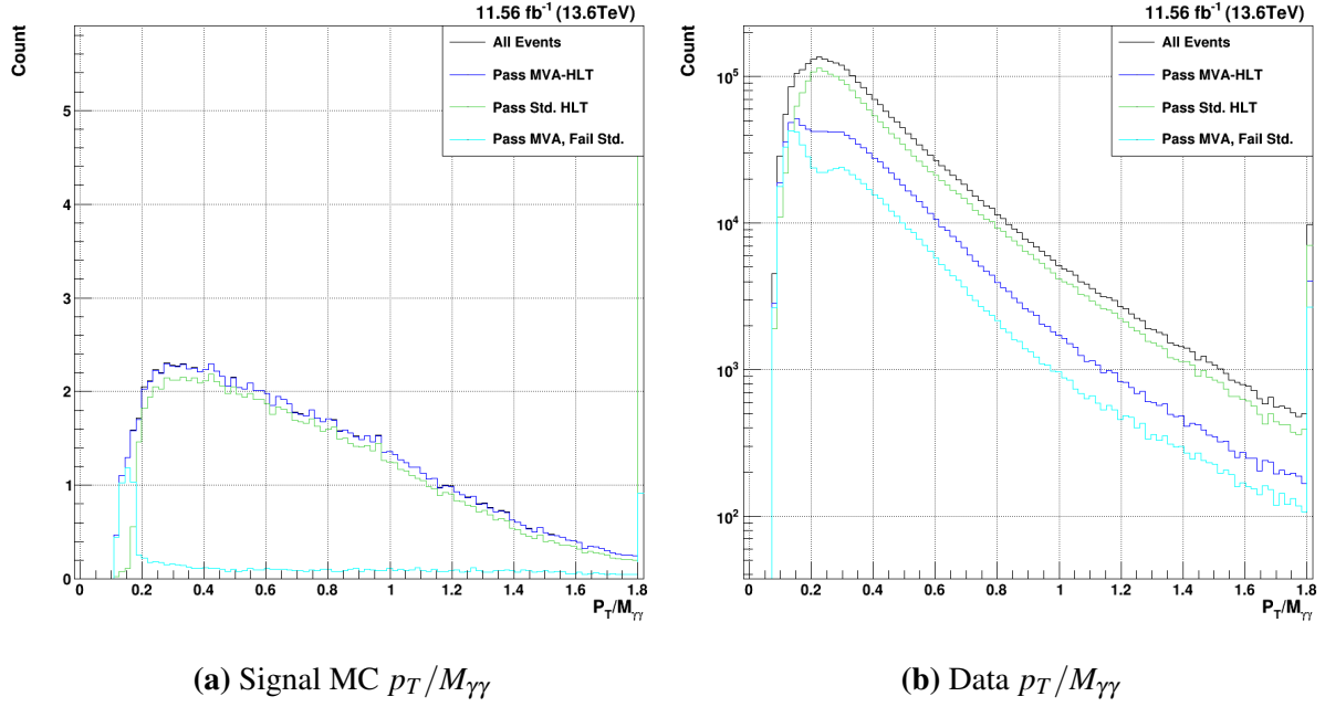
Figure 7.6. Acceptance of the MVA-HLT (blue) vs. the current standard diphoton HLT (green) for p_T/M_{\gamma\gamma}
