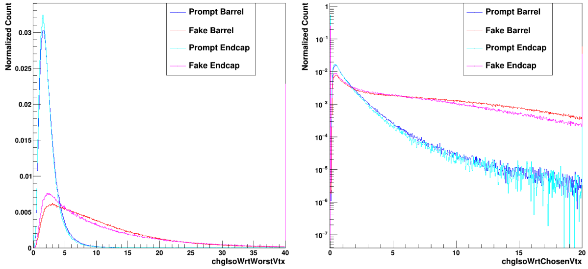
Figure 6.6. Plots of the charged isolations with respect to the chosen and worst vertices. The prompt signal is shown in dark blue for the barrel and light blue for the endcap, whereas the fake background is shown in red for the barrel and pink for the endcap.
