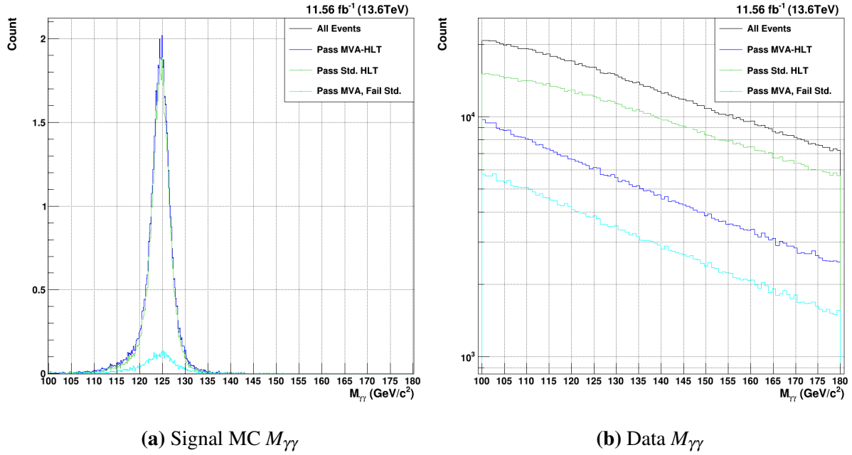
Figure 7.4. Acceptance of the MVA-HLT (blue) vs. the current standard diphoton HLT (green) for M_{\gamma\gamma}
