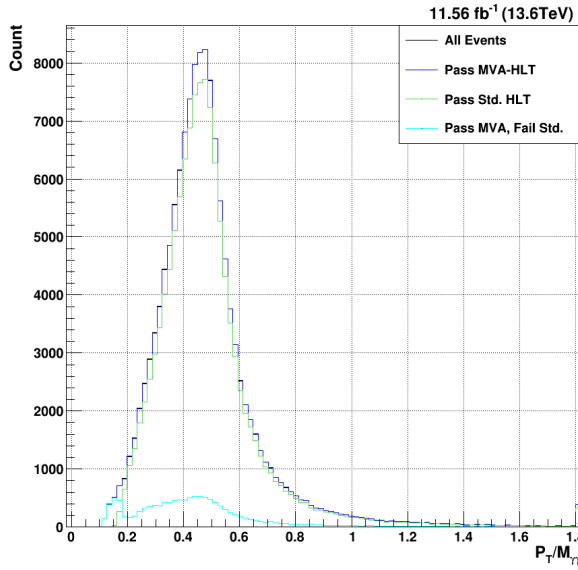
(a) Signal MC p_T/M_{\gamma\gamma}
