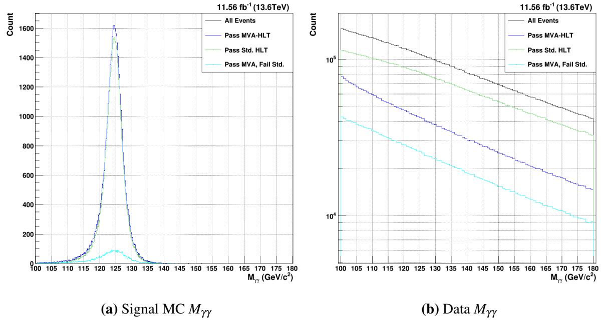
Figure 7.1. Acceptance of the MVA-HLT (blue) vs. the current standard diphoton HLT (green) for M_{\gamma\gamma}
