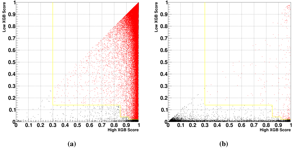
Figure 5.4. XGBoost output scores for two selected photon candidates in the Winter 2024 ggH signal MC (a), and 2023 Data (b). The higher of the two scores is plotted on the X-axis, while the lower of the two is plotted on the Y-axis.
